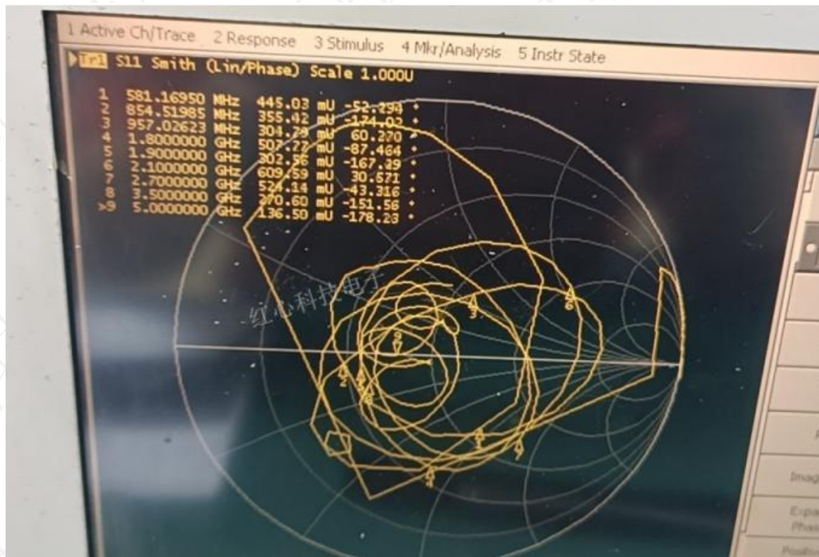
Smith Chart (史密斯圆图)
